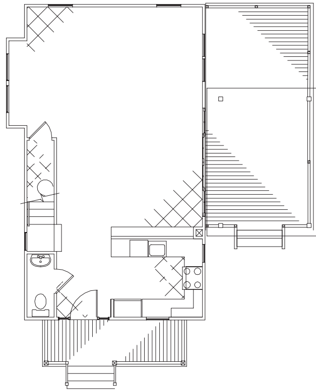
UNIT 18 - FIRST FLOOR PLAN
