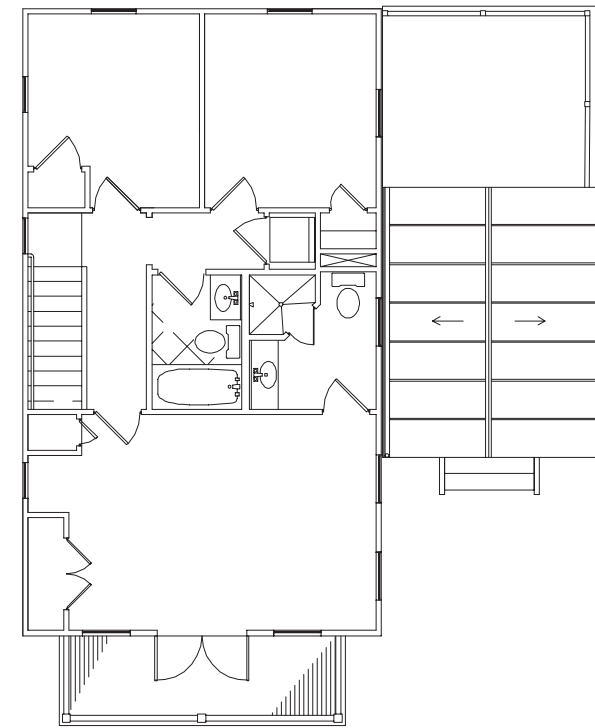
UNIT 18 - SECOND FLOOR PLAN
