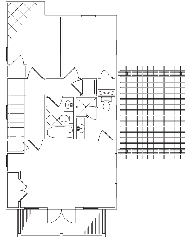
UNIT 20 - SECOND FLOOR PLAN
