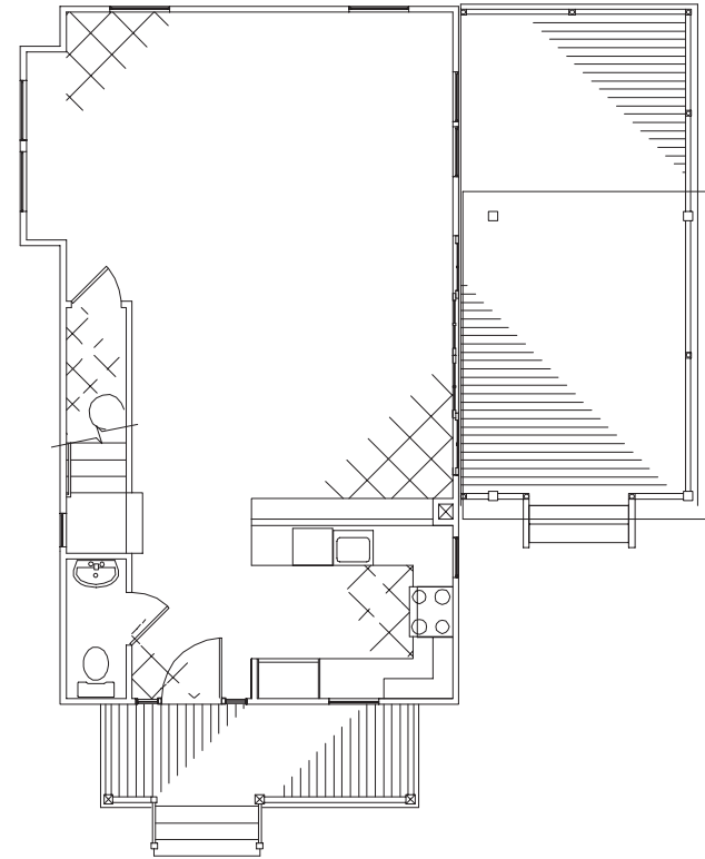
UNIT 20 - FIRST FLOOR PLAN
