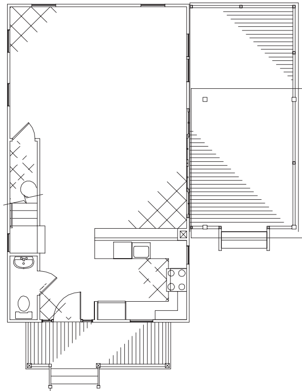
UNIT 22 - FIRST FLOOR PLAN
